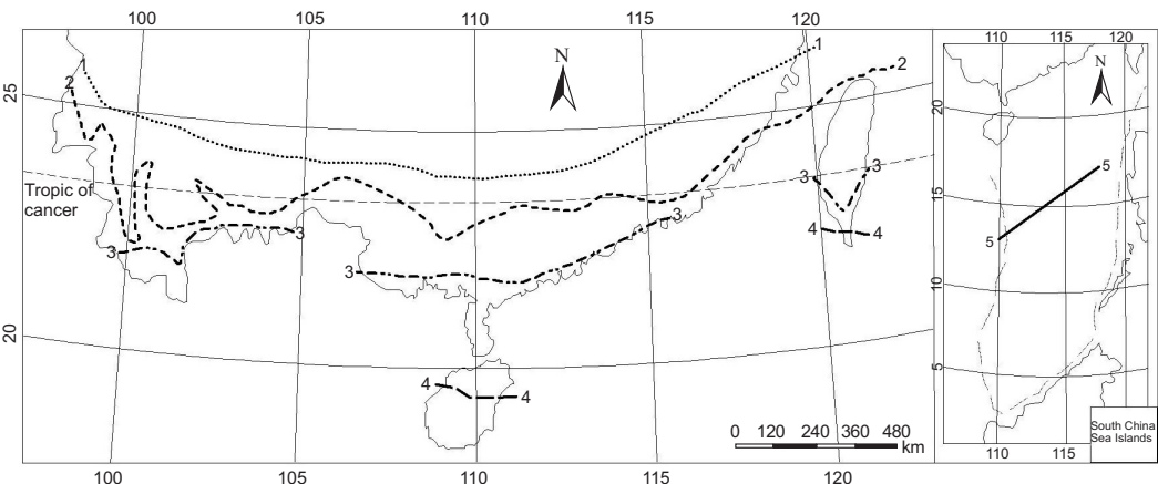
界线 1：主要依据广义热带植物分布的北界，大致在中国南部 24°~25°N、东南部达 26°N(福建)；界线 2：主要依据月均温 20°C 以上的天气达 8 至 11 个月；界线 3：主要依据 >10°C 有效年积温达 8000°C、最冷月均温 >16°C；界线 4：主要依据最低月均温 18°C、年生物温 25°C；界线 5：多用于赤道和热带的分界。 Line 1: Northern boundary of tropical zone in broad sense( without winter all year round) ; Line 2: Based on 8 – 11 months with monthly mean temperature over 20°C; Line 3: Based on effective accumulative temperature of 8000°C with >10°C daily mean temperature and mean temperature of coldest month >16°C; Line 4: Based on lowest monthly mean temperature of 18°C and annual biotemperature of 25°C; Line 5: Often used for equatorial and tropical boundaries.
