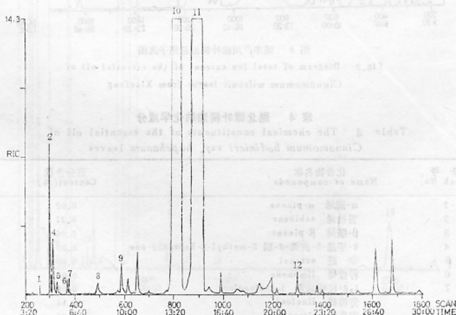
图 3 湖北樟叶精油总离子流图 Fig. 3 Diagram of total ion current of the essential oil of Cinnamomum bodinieri var. hupehanum leaves
